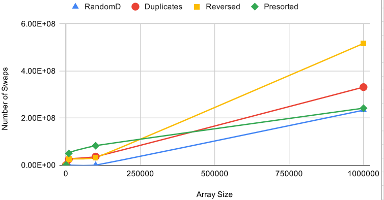
Quick Sort Number of Swaps
