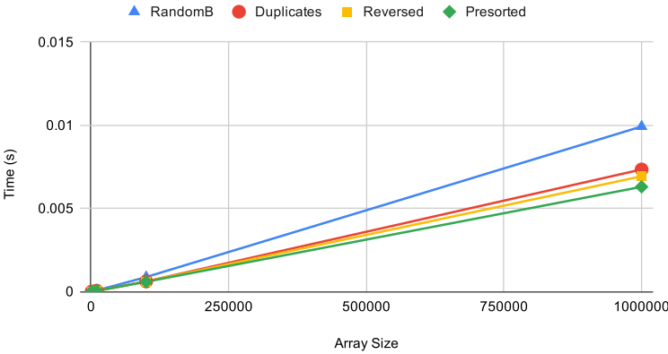
Merge Sort Time Complexity
