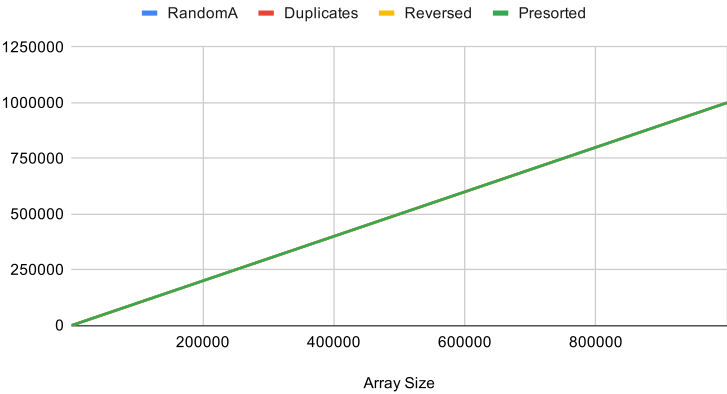
Merge Sort Comparisons
