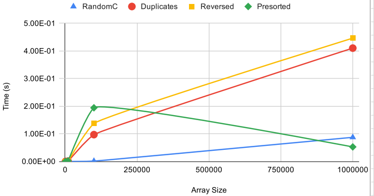
Quick Sort Time Complexity
